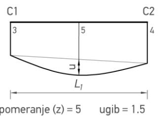
(f) Ivica terase C1 - C2
